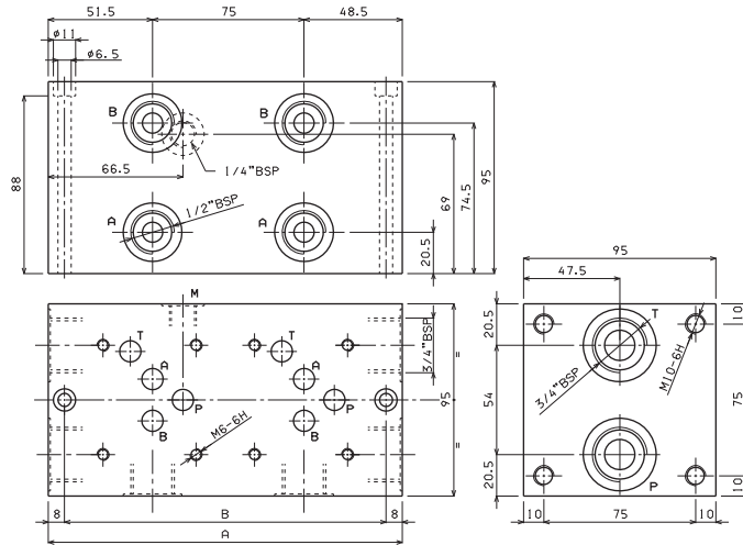
Fixing screws M6x100 UNI 5931
